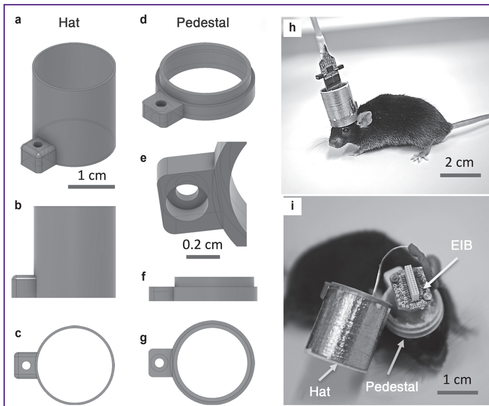
Design of 3D printed plastic parts for the HIME system: (a)–(g) 3D models made in Fusion 360 CAD software for printing with the 3D printer Ultimaker 2; (a)–(c) the protecting hat with a small hole ( \varnothing 2 mm) for the 10 mm M1 screw to be used to hold the hat on the bottom pedestal; (d)–(g) the bottom pedestal which is supposed to be fixed with dental cement on the mouse head; (e) magnified view of the pedestal bottom part depicting a bigger hole ( \varnothing 3 mm) for insertion a female screw for the M1 male screw, which is fixed there by melting plastic around with a hot soldering tip; (h) an example of implanted mouse bearing electrodes, 3D printed plastic parts and connected with a 16 channels Neuralynx preamplifier with a long tether/cable; (i) an awake mouse with the removed protecting hat exposing Neuralynx EIB-18, golden pins, electrodes, a ground wire and the dental acrylic fixed to the mouse cranium bone bottom pedestal
