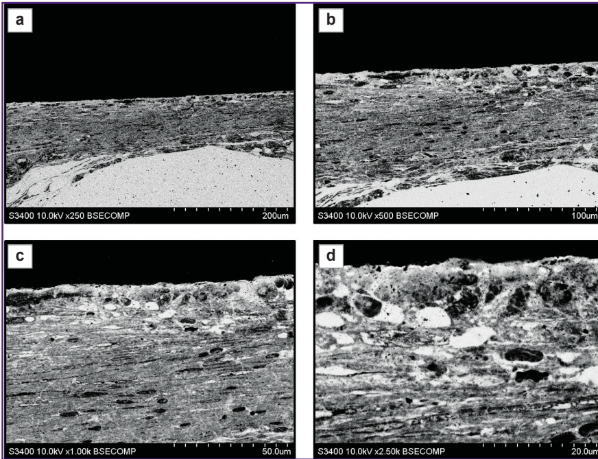
Figure 2. Perforated plate made of patented original titanium alloy, removed 2 months after intracranial implantation to New Zealand white rabbits Visualization of the barrier between the plate and tissues ((a) \times 250 ; (b) \times 500 ) and differentiation of connective tissue into two layers: (c) underlying dense layer containing elongated cells with oblong nuclei, \times 1000 ; (d) the layer adjacent to the plate, loose with rounded intercellular spaces, \times 2500
