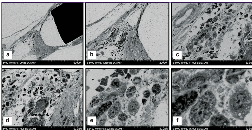
Figure 3. Perforated plate made of patented original titanium alloy, removed 1 month after intracranial implantation to New Zealand white rabbits Connective tissue capsule forming around the plate: (a) general view of the plate with surrounding tissues, \times 100 ; blood vessels and multiple cells of the surrounding tissue: (b) \times 250 ; (c) \times 1000 ; numerous macrophages in the focus of productive inflammation: (d) \times 1000 ; (e) \times 2500 ; (f) \times 5000
