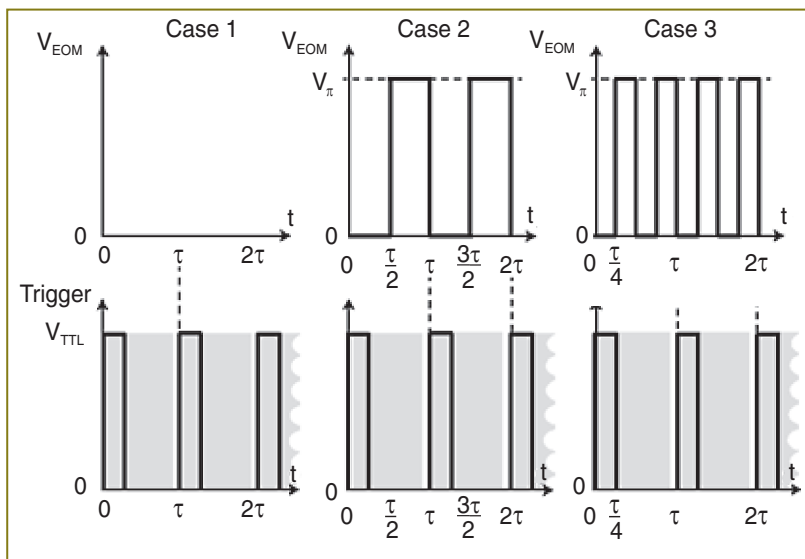
Figure 1. Phase shifting schemes. Case 1: no phase shift. Case 2: \pi -phase shift during half the A-scan exposure time. Case 3: two \pi -phase shifts during one A-scan exposure time. The time trace above is the EOM driving voltage with V_\pi being the half-wave voltage. The trace below is the camera trigger signal. The shaded area denotes the time of exposure assuming a better than 90% duty cycle
