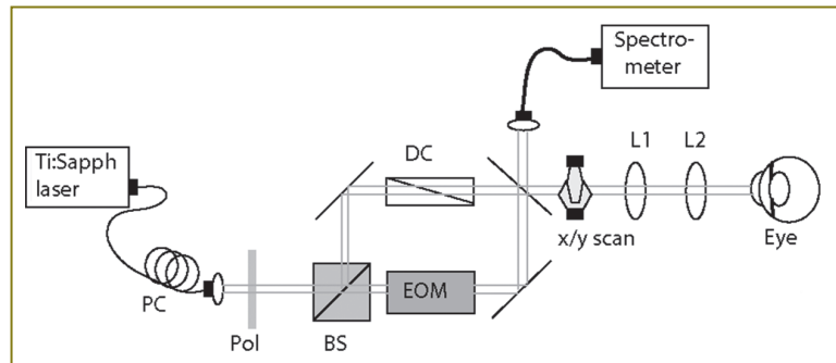
Figure 5. Optical setup (PC — polarization controller; Pol — polarizer; BS — 50:50 beam splitter; DC — dispersion control; EOM — electro-optic-modulator; L1, L2 — achromats)
