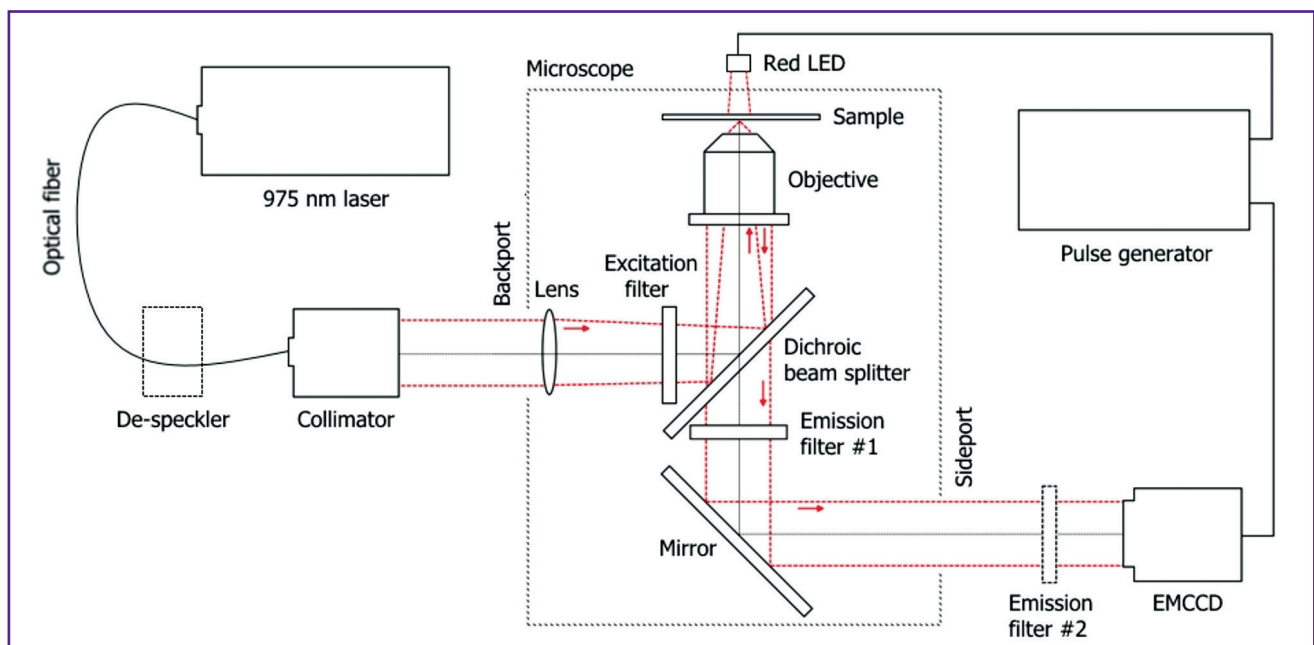
Figure 1. The scheme of the experimental setup for upconversion nanoparticles tracking in living cells
