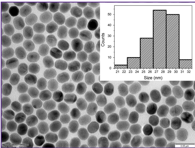
Figure 2. The transmission electron microscopy image of \text{NaYF}_4:\text{Yb,Tm} nanoparticles
