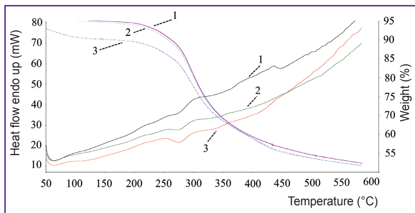
Figure 2. Temperature dependence of mass loss and thermal effects:
