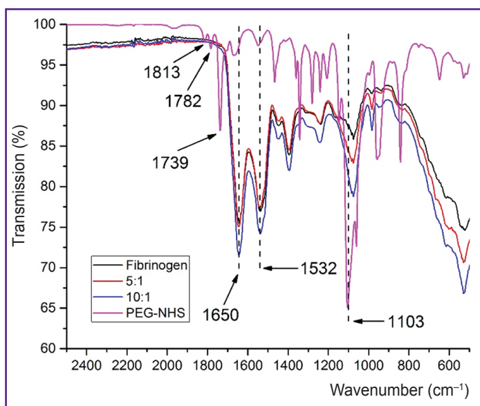
Figure 1. Fourier transform infrared spectra of pure fibrinogen, NHS-functionalized polyethylene glycol (PEG-NHS) and PEGylated fibrinogen with molar ratios 5:1 and 10:1
